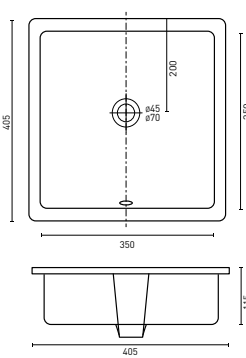
CARINA - Square (p. 52) 405 x 405 x 175 [6.4L]
