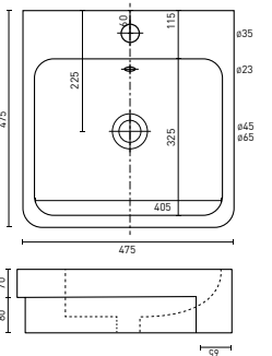
NOVARA - Rectangle (p. 53) 475 x 475 x 150 [6L]
