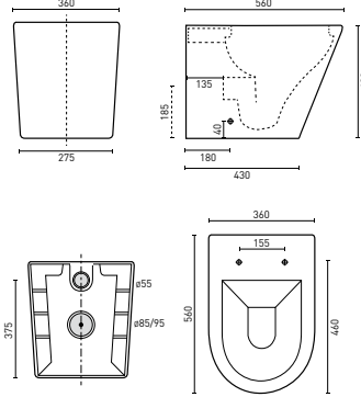
RENEE RIMLESS WALL FACED PAN (p. 47) 560 x 360 x 420 mm - Universal set out 60-90mm
