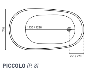
PICCOLO (P. 8) 1500 x 740 x 700 mm (127L) 1700 x 740 x 700 mm (167L)
