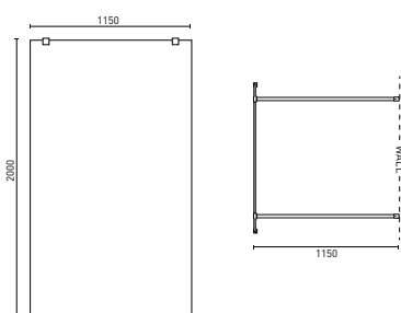
M-SERIES FREESTANDING (P. 35) 1150 x 2000 mm
