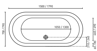
COOL (P. 5) 1500 x 750 x 580 mm (140L) 1790 x 790 x 580 mm (155L)
