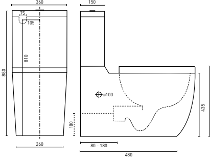
ALEGRA EZI HEIGHT RIMLESS BACK-TO-WALL (p. 44) 635 x 360 x 880 mm - Universal set out 60-180mm
