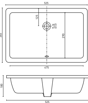
SAN DIEGO - Rectangle (p. 52) 525 x 345 x 180 [7L]
