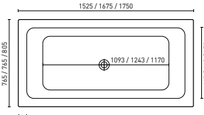
CARINA (P. 17) 1525 x 765 x 440 mm (147L) 1675 x 765 x 440 mm (166L) 1750 x 805 x 480 mm (182L)
