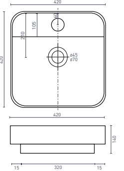
CARINA - Square (p. 39) 420 x 420 x 140 [7.8L]
