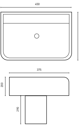
ARIA - Rectangle (p. 54) 450 x 375 x 200 [4.5L]
