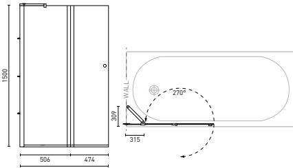
CASCADE FIXED & SWING PIVOT PANEL BATH SHOWER SCREEN (p. 39) 1037 x 1500mm - swings 270°
