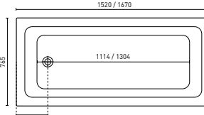
CORTEZ (P. 17) 1520 x 765 x 450 mm (136L) 1670 x 765 x 450 mm (154L)
