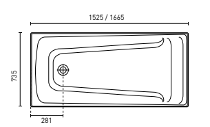
NOVARA INSET (P. 17) 1525 x 735 x 447 mm (101L) tile bead 1665 x 735 x 447 mm (114L) tile bead
