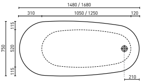
CAVAL (P. 5) 1480 x 750 x 680 mm (129L) 1680 x 750 x 680 (150L)
