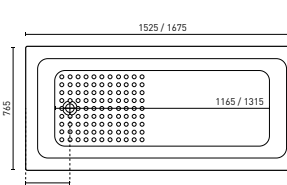
FABRINO (P. 17) 1520 x 765 x 400 mm (130L) 1675 x 765 x 400 mm (154L)
