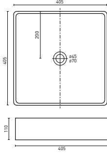
CARINA - Square (p. 50) 405 x 405 x 110 (9.5L)
