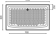
AZZURO (P. 19) 1200 x 820 x 425 mm (116L)
