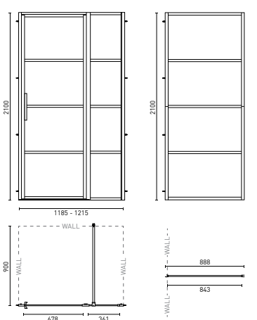
MANHATTAN (P. 38) 1200 x 2100 mm 900 x 2100 mm (return panel)
