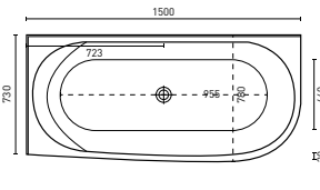
NATALIA (P. 11) 1500 x 780 x 550 mm (125L)
