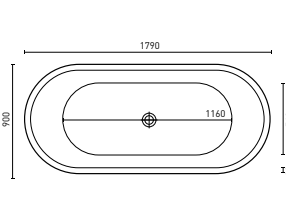
MINTORI (P. 6) 1790 x 900 x 596-630 mm (190L)
