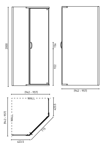
CASCADE ANGLE (P. 37) 940 x 940 x 2000 mm
