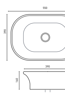
LOLA - Oval / Rectangle (p. 51) 550 x 390 x 160 (7.5L)
