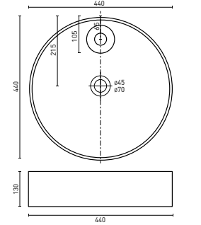
CAVAL - Round (p. 50) 440 x 440 x 130 (6L)
