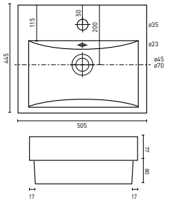
NOVARA - Square (p. 52) 505 x 445 x 157 [6L]
