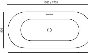
VALENTINA (P. 9) 1500 x 800 x 600 mm (165L) 1700 x 800 x 600 mm (176L)
