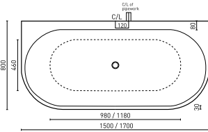
ALEGRA (P. 12) 1500 x 800 x 590 mm (162L) 1700 x 800 x 590 mm (175L)
