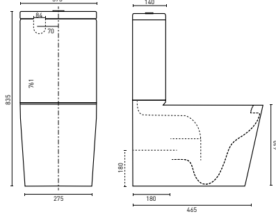
FABRINO RIMLESS BACK-TO-WALL (p. 44) 610 x 373 x 835 mm - Universal set out 90-180mm
