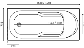
ADATTO (P. 16) 1510 x 715 x 445 mm (106L) 1650 x 715 x 445 mm (122L)
