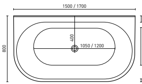
ALEGRA (P. 11) 1400 x 800 x 600 mm (135L) 1500 x 800 x 600 mm (162L) 1700 x 800 x 600 mm (175L)
