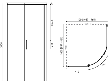
FLORIANO (P. 37) 957 x 957 x 2000 mm
