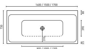
BIANCO (P. 11) 1400 x 730 x 550 mm (150L) 1500 x 730 x 550 mm (170L) 1700 x 730 x 550 mm (200L)
