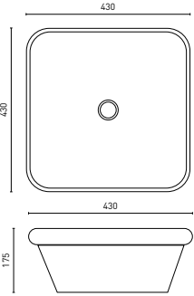
CARINA - Square (p. 39) 430 x 430 x 175 [5.2L]
