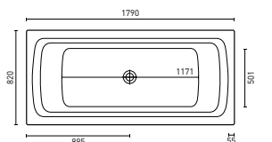
SAN DIEGO (P. 18) 1790 x 820 x 480 mm (194L)
