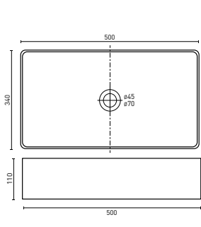
SAN DIEGO - Rectangle (p. 51) 500 x 340 x 110 (10.3L)
