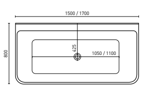
ARIA (P. 11) 1500 x 800 x 610 mm (182L) 1700 x 800 x 600 mm (201L)
