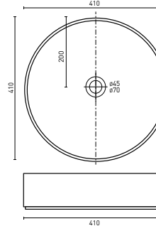
CAVAL - Round (p. 50) 410 x 410 x 125 (10L)
