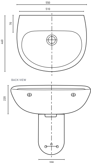
NOVARA - oval (p. 54) 550 x 460 x 220 [7.5L]
