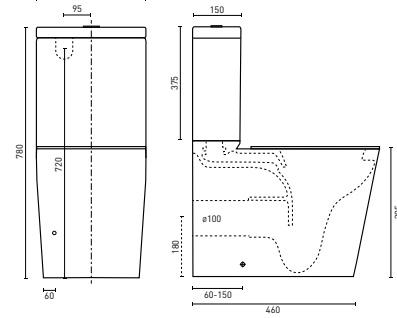
PREZZO RIMLESS BACK-TO-WALL (p. 45) 615 x 380 x 780 mm - Universal set out 60-150mm
