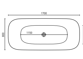
LOLA (P. 6) 1700 x 800 x 600 mm (198L)
