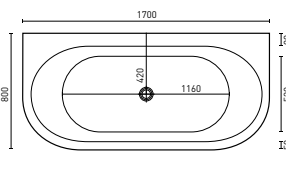
OXFORD (P. 11) 1700 x 800 x 600 mm (174L)
