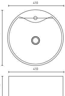
CAVAL - Round (p. 50) 410 x 410 x 145 (7.5L)
