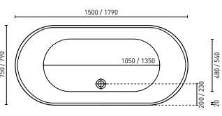
ELINEA (P. 6) 1500 x 750 x 580 mm (150L) 1790 x 790 x 570 mm (200L)
