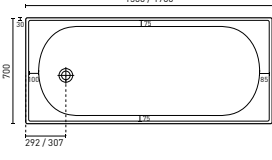
GIORGIA (P. 19) 1500 x 700 x 360 mm (65L) 1700 x 700 x 360 mm (75L)
