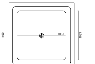
VENICE (P. 18) 1400 x 1400 x 500 mm (370L)
