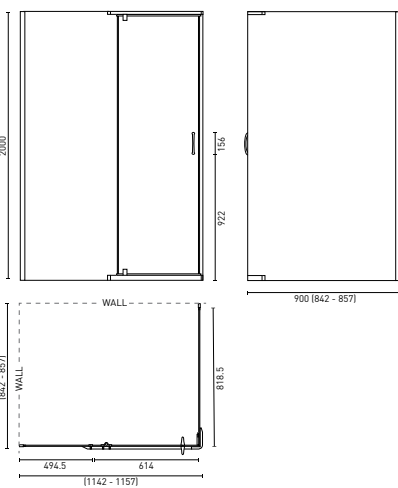
CASCADE RECTANGLE (P. 36) 1140 x 840 x 2000 mm
