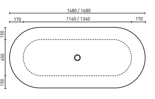
NOVARA (P. 7) 1480 x 750 x 580 mm (139L) 1680 x 750 x 580mm (182L)
