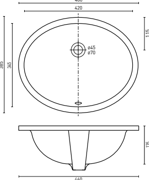
NOVARA - Oval (p. 52) 460 x 385 x 190 [5.2L]
