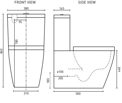
RENEE EZI HEIGHT RIMLESS BACK-TO-WALL (p. 45) 643 x 380 x 845 mm - Universal set out 60-180mm
