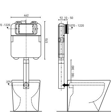
WALL FACED INWALL CISTERN (p. 47) 462 x 92 x 570 mm - Universal set out 60-90mm
