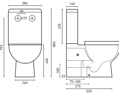
ADATTO EZI HEIGHT RIMLESS BACK-TO-WALL (p. 44) 660 x 380 x 840 mm - Universal set out 90-180mm
