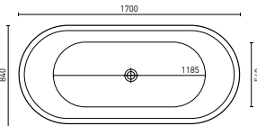
ELISI (P. 13) 1700 x 840 x 595 mm (190L)
