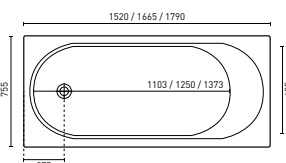
TURIN (P. 18) 1520 x 755 x 445 mm (121L) 1665 x 755 x 445 mm (138L) 1790 x 755 x 485 mm (153L)
