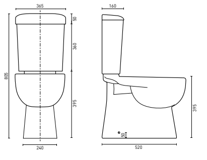
NOVARA RIMLESS CLOSED COUPLED (p. 44) 640 x 375 x 805 mm - S-Trap set out 140
