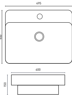
ARIA - Rectangle (p. 39) 495 x 400 x 150 [5.2L]
