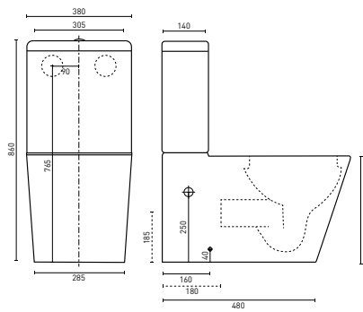
RENEE RIMLESS BACK-TO-WALL (p. 45) 615 x 380 x 860 mm - Universal set out 60-150mm
