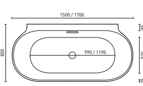
AURORA (P. 11) 1500 x 800 x 600 mm (135L) 1700 x 800 x 600 mm (162L)
