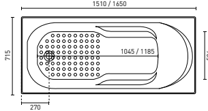
BAMBINO (P. 17) 1510 x 715 x 380 mm (88L) 1650 x 715 x 380 mm (103L)
