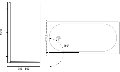
FITROY PIVOT PANEL BATH SHOWER SCREEN (p. 39) 800 x 1500mm
