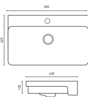
ARIA - Rectangle (p. 53) 500 x 420 x 130 [7.5L]
