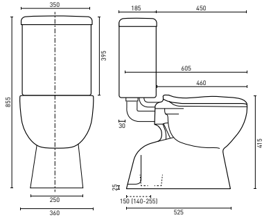
NOVARA CONNECTOR (p. 44) 685 x 350 x 855 mm - S-Trap set out 140-165mm
