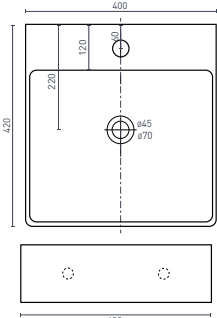
ARIA - Square (p. 50) 400 x 420 x 155 (4.5L)
