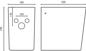
ARIA - Shroud (p. 54) 180 x 300 x 290
