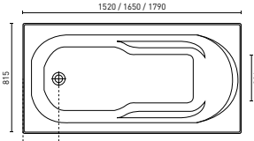
PRIMA (P. 18) 1515 x 815 x 445 mm (124L) 1635 x 815 x 510 mm (159L) 1785 x 815 x 510 mm (194L)
