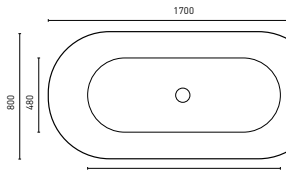
SOLIS (P. 9) 1700 x 800 x 580 mm (135L)
