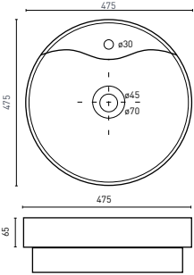
CAVAL - Round (p. 39) 475 x 475 x 135 [6L]
