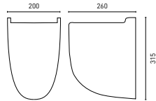
NOVARA - Shroud (p. 54) 200 x 260 x 315
