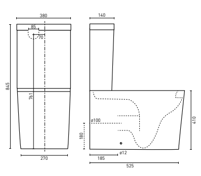
SAN DIEGO RIMLESS BACK-TO-WALL (p. 45) 640 x 380 x 845 mm - Universal set out 90-180mm
