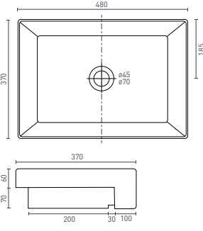
SAN DIEGO - Rectangle (p. 53) 480 x 370 x 130 [13L]
