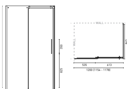
AVALON / MALANDA (P. 36) 1154 x 854 x 2000 mm 1200 x 900 x 2000 mm
