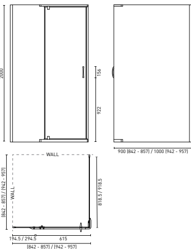
CASCADE SQUARE (P. 36) 840 x 840 x 2000 mm 940 x 940 x 2000 mm
