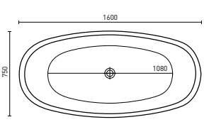
SHERATON (P. 9) 1600 x 750 x 410 mm (125L)
