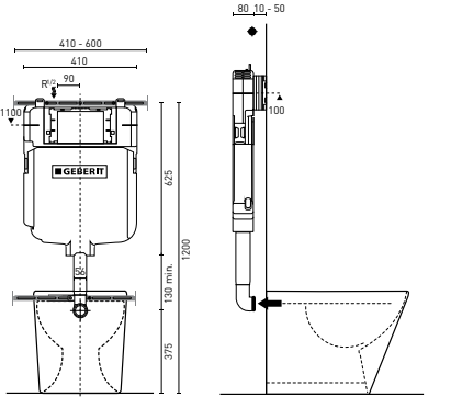
GEBERIT WALL FACED INWALL CISTERN (p. 47) 410 x 80 x 625 mm - Universal set out 60-90mm
