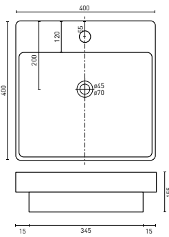
ARIA - Square (p. 39) 400 x 400 x 155 [4.5L]
