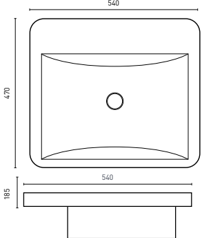
SAN DIEGO - Rectangle (p. 53) 540 x 470 x 185 [7.5L]
