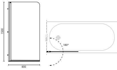
CASCADE PIVOT PANEL BATH SHOWER SCREEN (p. 39) 790 x 1500mm - swings 180°
