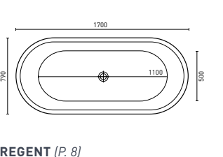
REGENT (P. 8) 1700 x 790 x 600 mm (250L)
