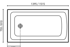
SHENSEKI (P. 18) 1395 x 755 x 480 mm (137L) 1515 x 810 x 520 mm (191L)
