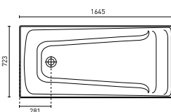
NOVARA ISLAND (P. 18) 1645 x 723 x 435 mm (114L) NO tile bead
