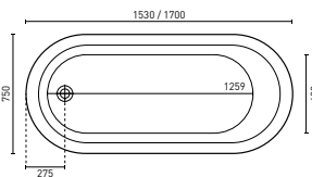
UNO (P. 18) 1530 x 750 x 480 mm (140L) 1700 x 750 x 490 mm (168L)
