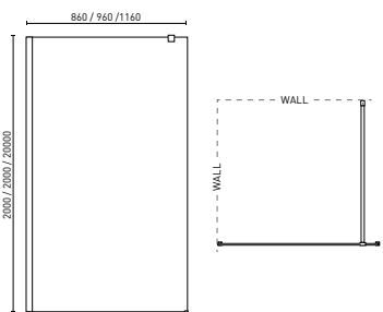
M-SERIES WALL FIXED (P. 34) 860 x 2000 mm 960 x 2000 mm 1160 x 2000 mm
