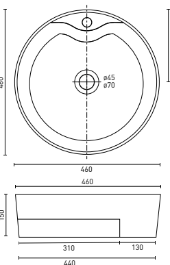
CAVAL - Round (p. 53) 460 x 460 x 150 [5L]
