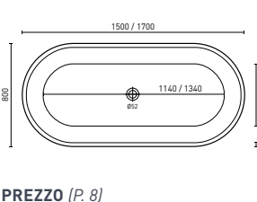
PREZZO (P. 8) 1500 x 800 x 530 mm (121L) 1700 x 800 x 530 mm (150L)
