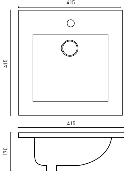
CARINA - Square (p. 53) 415 x 415 x 170 [4.5L]
