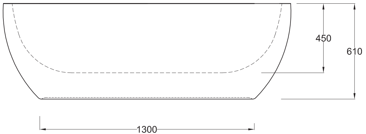
FRONT VIEW
